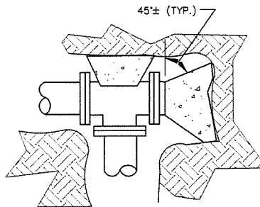
TEE (PLUGGED)
