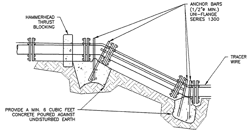
VERTICAL BEND DETAIL
